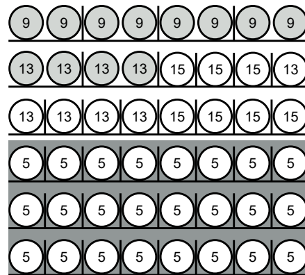
6 double spirals, 36 single spirals 2 temperature zones
